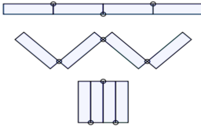
Figure 1 Axis Shift Fold (offset fold line)
