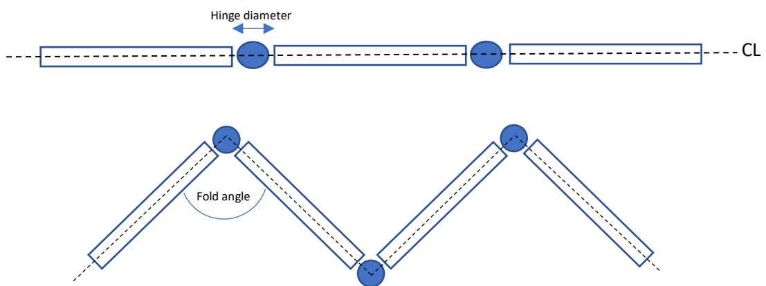
Figure 2 Ideal fold line (material thickness centreline not shifted)
